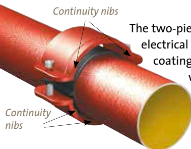
Two-piece ductile iron couplings
