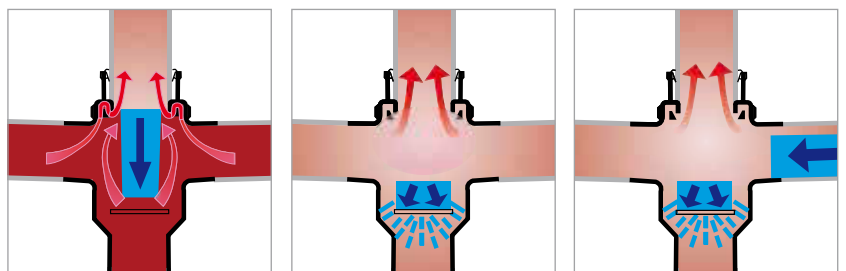
Inside the branch, at the bottom of the body, a rubber deflector sprays the column of water to prevent draught or self siphonage.
