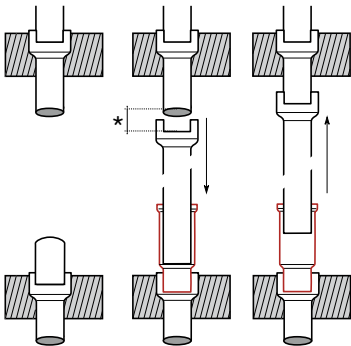
Slip fitting Vertical lift required = 220 mm
