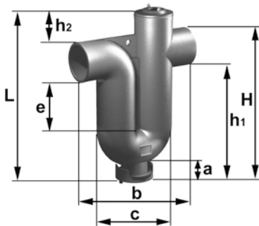
Plus range trap DN 50 to 150
