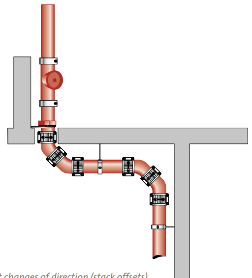
At changes of direction (stack offsets).
