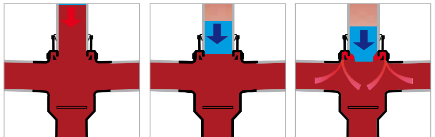
Owing to the special design of the branch, after a flush, the column of water is directed so that air can pass over the flow and naturally vent the stack.
