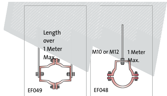
Typical support arrangement for horizontal pipework
