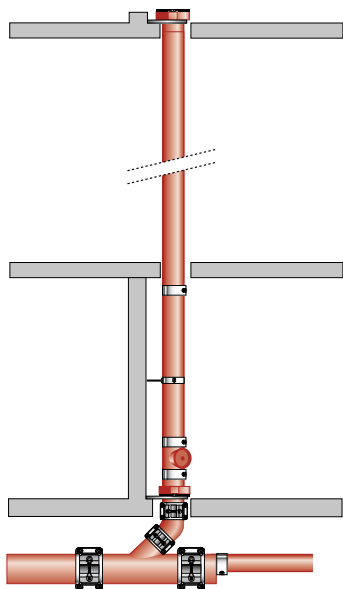
At the bottom of the stack
