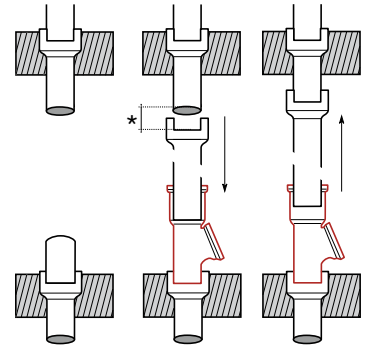
Slip branch Vertical lift required = 280 mm
