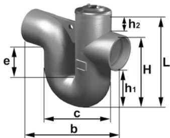
Plus range trap DN 200
