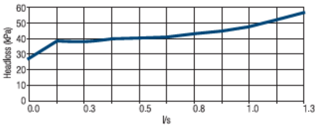
Double Check Assembly 15mm
