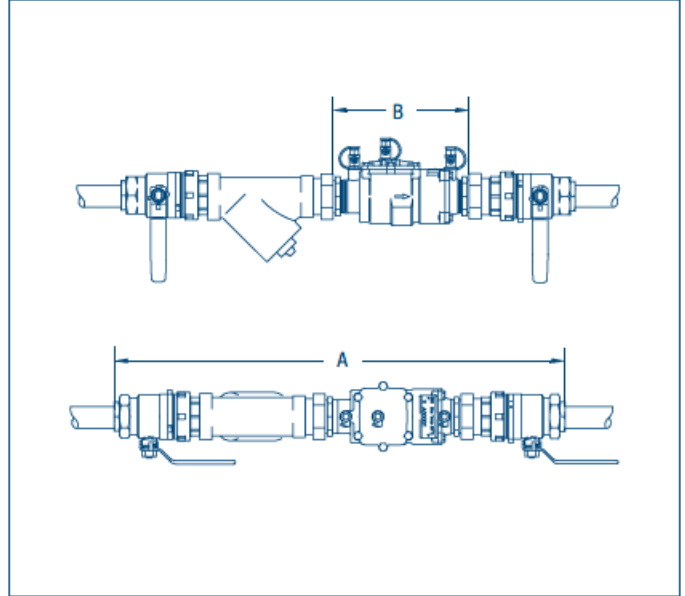
Double Check Assembly 32mm
