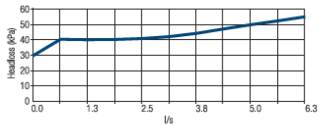
Double Check Assembly 32mm
