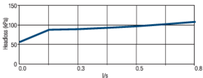
Reduced Pressure Assembly
