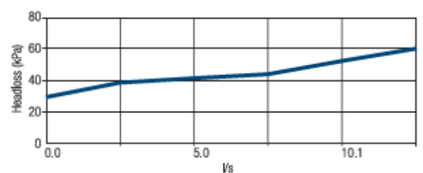
Double Check Assembly 50mm
