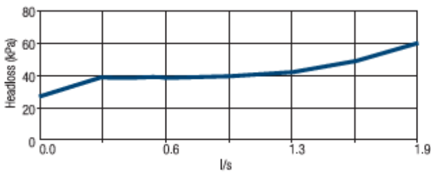
Double Check Assembly 20mm
