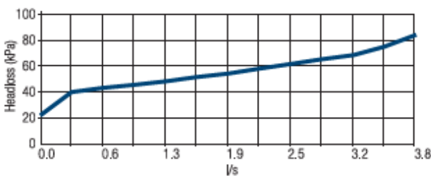
Double Check Assembly 25mm
