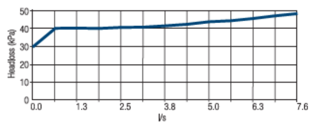
Double Check Assembly 40mm
